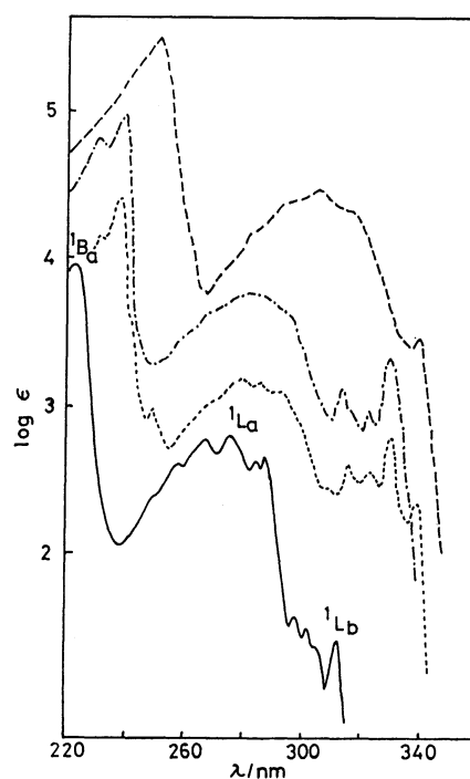
Fig. 1. The UV spectra for — naphthalene, ---- 1,2,3,7-tetramethyl- ( 10 ), ..... 2,7-dimethyl- ( 14 ), and —·—·— 1,3,6,8-tetramethyl-1,2,3,3a,4,5-hexahydropyrenes ( 18a , 18b , and 18c ) determined in cyclohexane. Absorption, log \epsilon , is for compound 10 .
